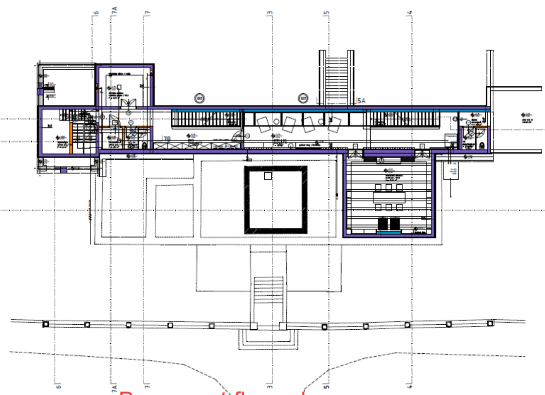
Basement floor plan V0_TLOCRT PODRUMA
